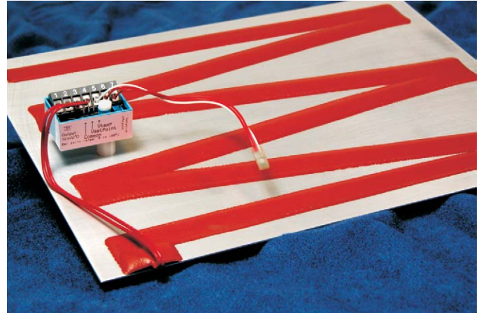
This Minco expanded heater assembly includes a temperature sensor and control electronics.
