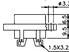
PANEL CUT-OUT
