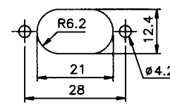
PANEL CUT-OUT
